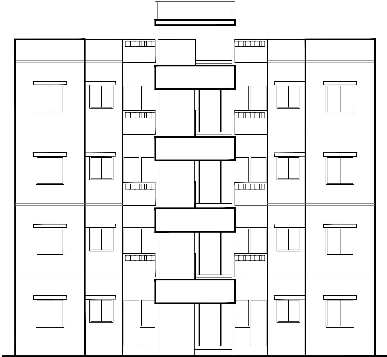
TYPICAL ROW HOUSING FRONT ELEVATION OF CLUSTERS
